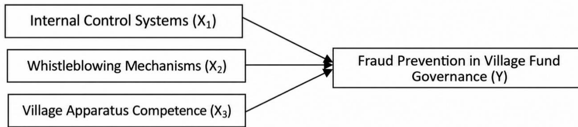
Figure 1. Research Framework
